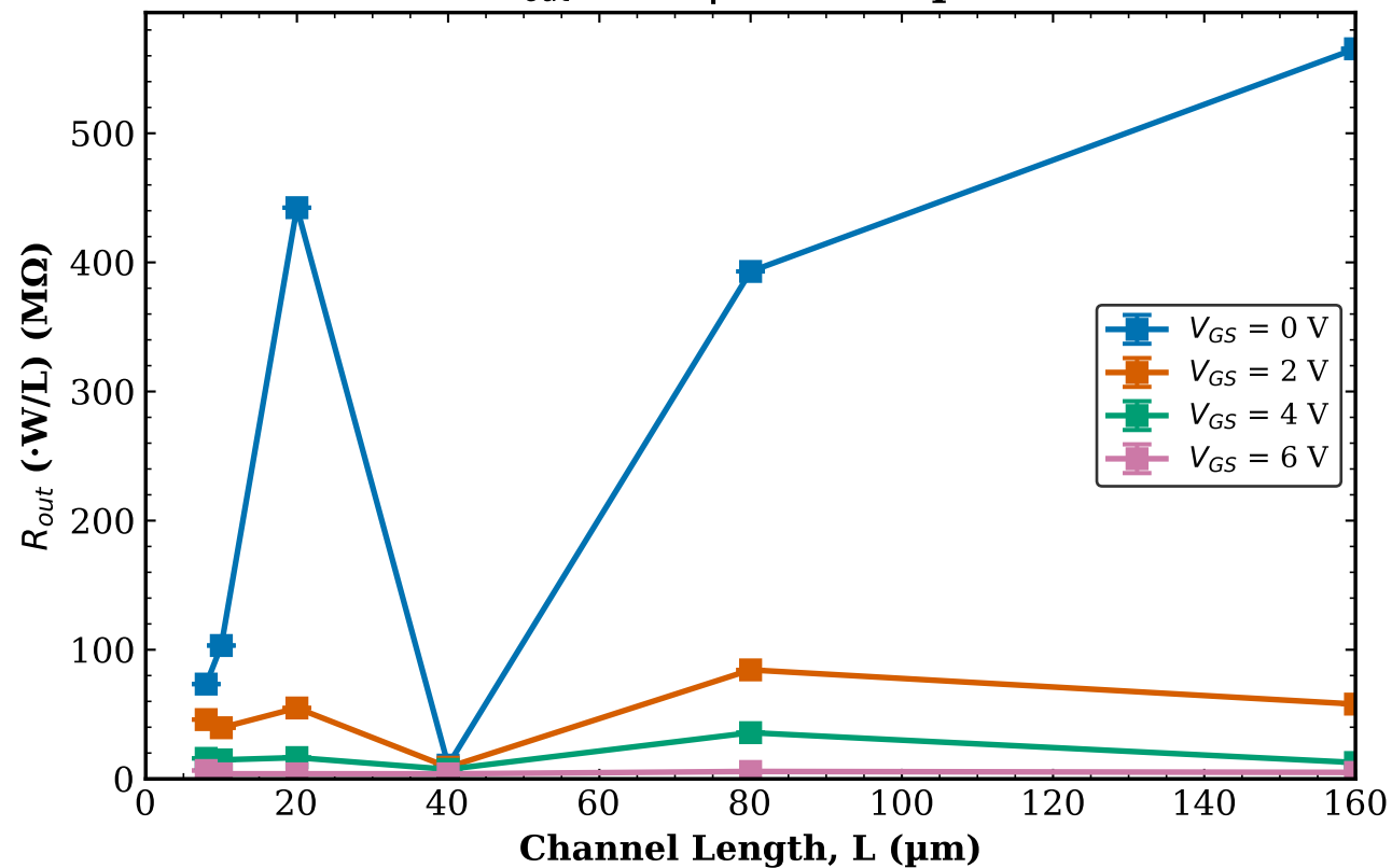
TFT3 Transistor 2 R_{out} vs L | W = 10\text{ }\mu\text{m}
